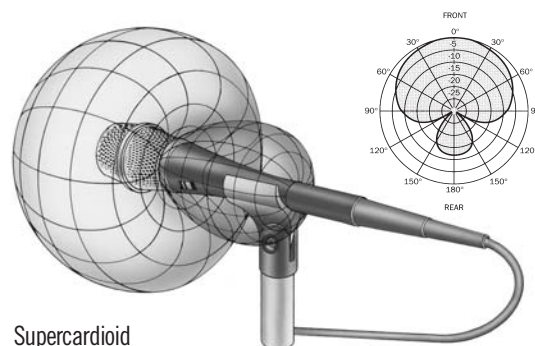
Cardioid (unidirectional)
