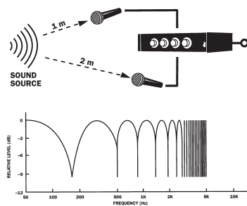
Multi-mic comb filtering
